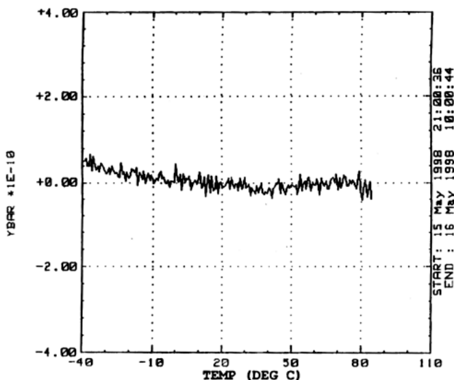
Figure 6 Frequency vs Temperature, FE-5652A
